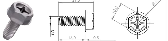
PF 30 - Parafuso Universal
